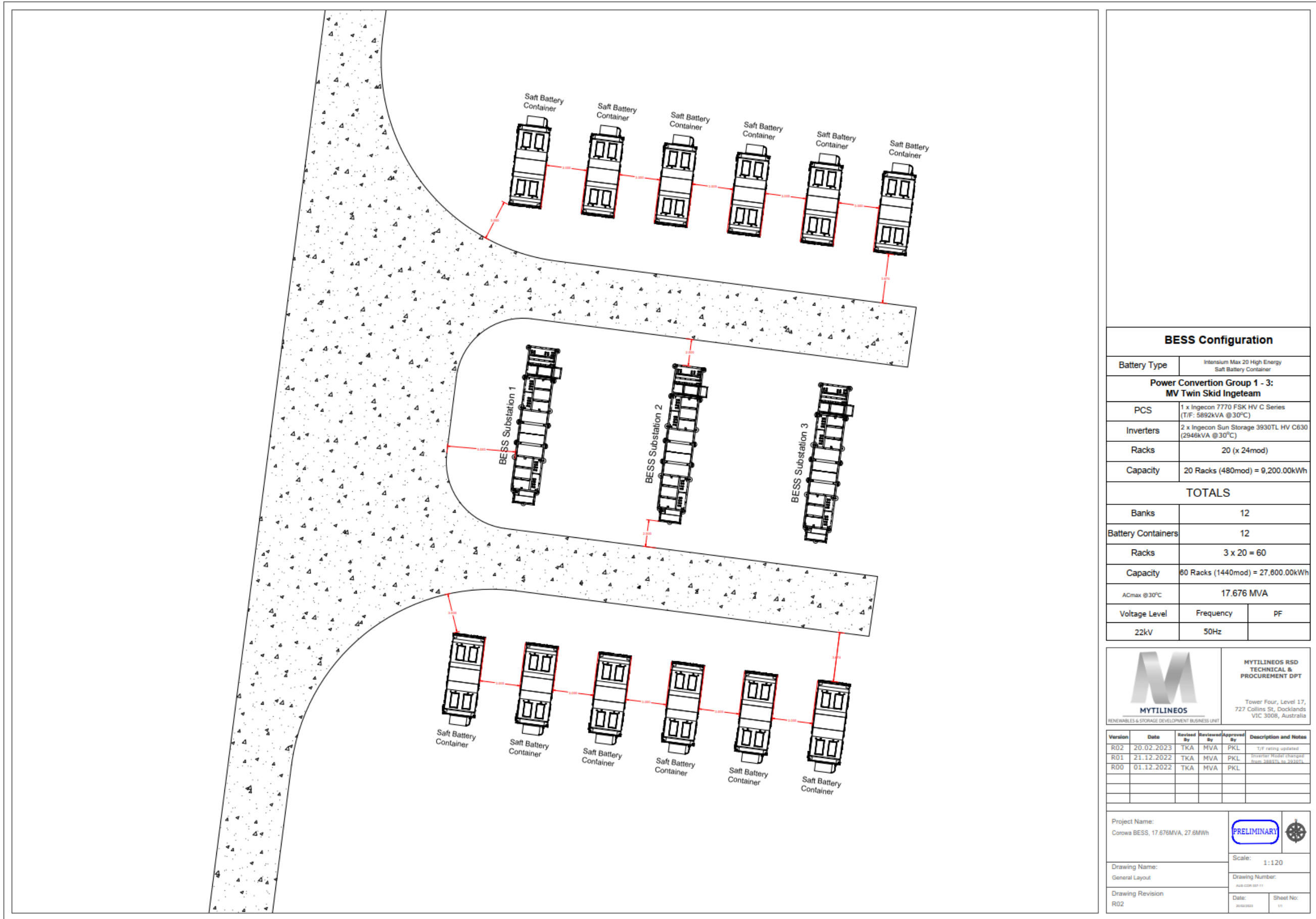
Figure 3-3: BESS Layout
